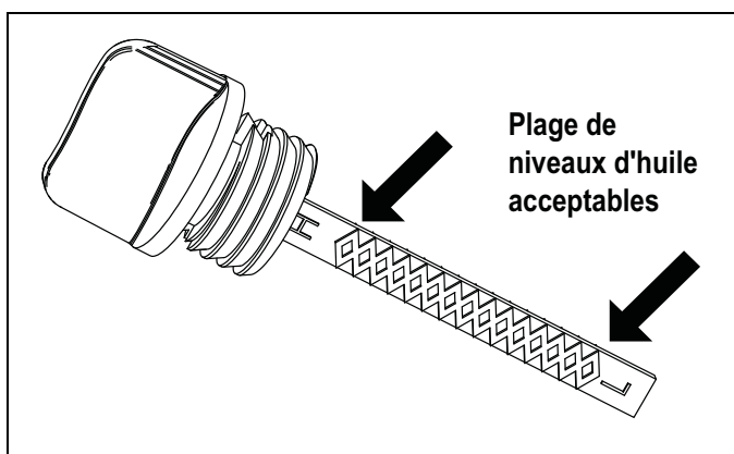
Figure 4-4. Jauge
