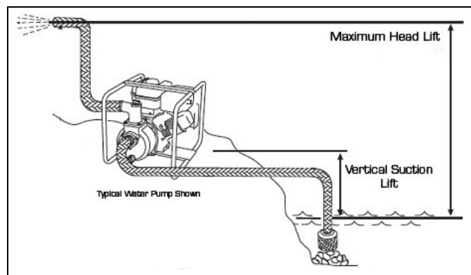
Figure 5-2. Pump Output
